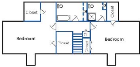
SECOND FLOOR
